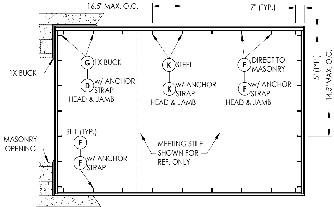
FRAME ANCHORING (1X, Steel Stud, Direct to Masonry)
