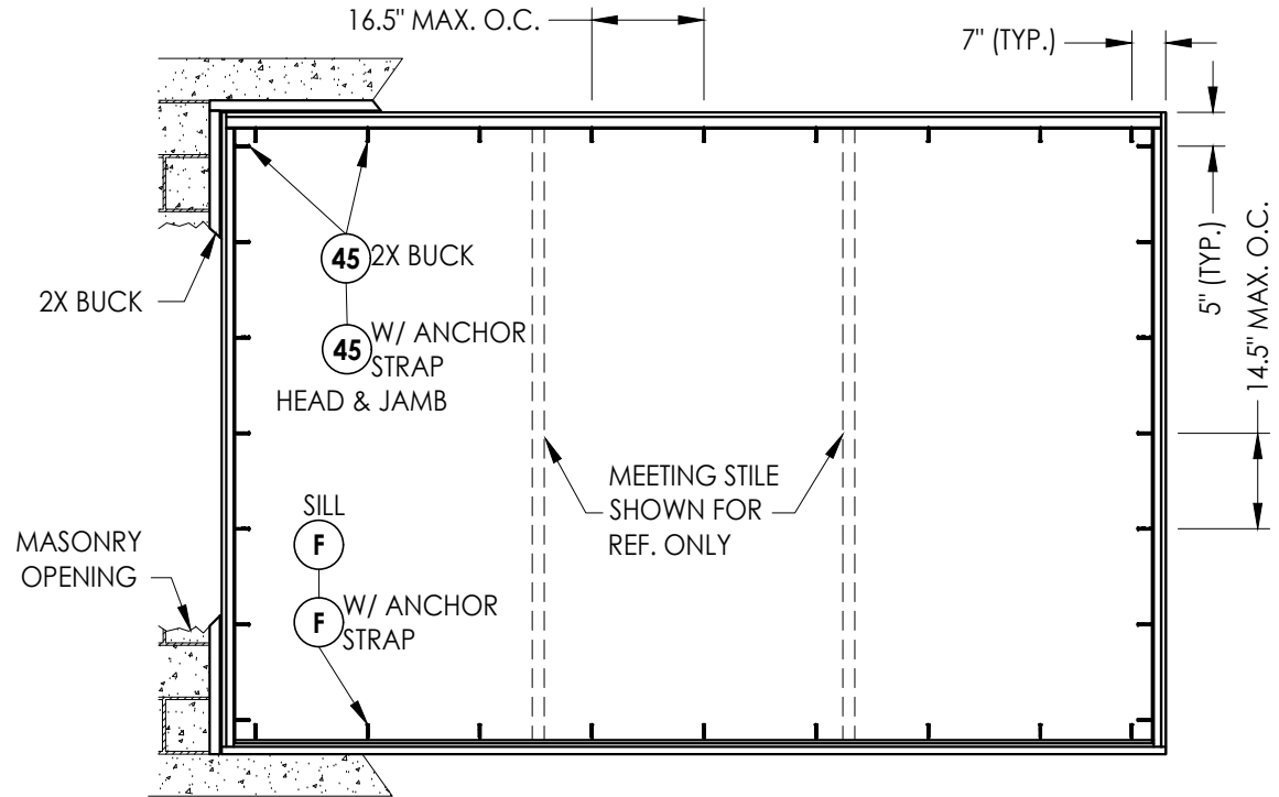
FRAME ANCHORING 2X
